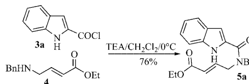
Scheme 1. Synthesis of pyrazino-indol-1-one precursor 5a .
