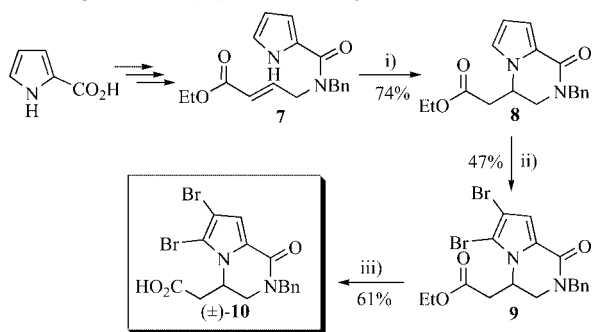
Scheme 4. Racemic synthesis of N -Bn-longamide b. Reagents and conditions: i) K_2CO_3 (10 mol-%), DMSO, room temp., 20 min; ii) NBS, CH_2Cl_2 , room temp.; iii) KOH, MeOH/ H_2O , reflux, 16 h.
