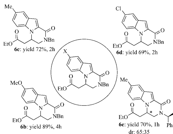
Scheme 2. Catalytic synthesis of functionalized dihydropyrazino[1,2- a ]indol-1(2 H )-ones.
