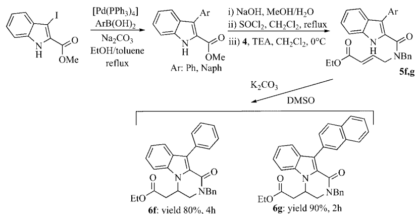
Scheme 3. Synthesis of 3-aryl-dihydropyrazino-indolinones 6f,g by K_2CO_3 -catalyzed ring-closing reaction.
