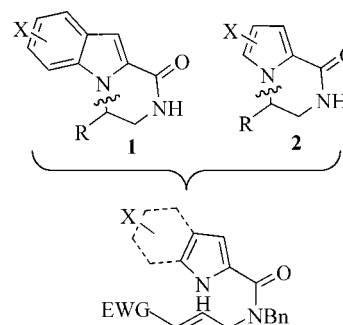
Figure 1. Intramolecular Michael addition as a key step in the synthesis of polycyclic indole- and pyrrole-based compounds.
