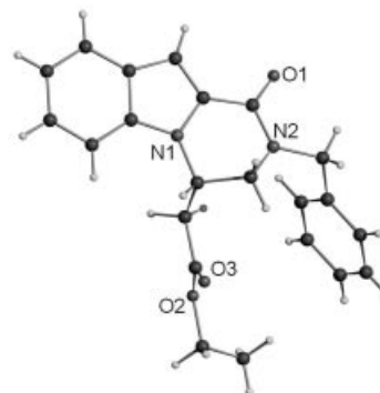
Figure 2. X-ray structure of (±)- 6a (only one enantiomer is shown).
